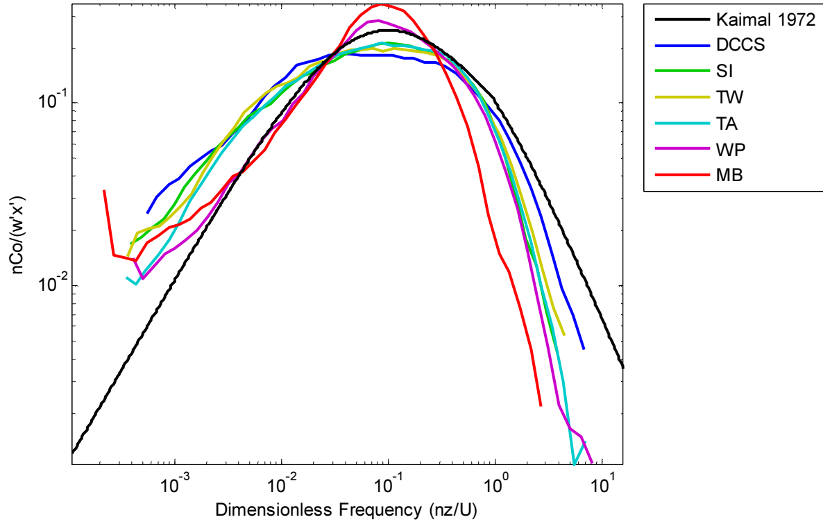
Median wC Unstable Cospectra - 24 May to 12 June 2013
