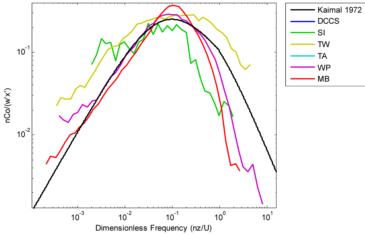
Median wM Unstable Cospectra - 24 May to 12 June 2013
