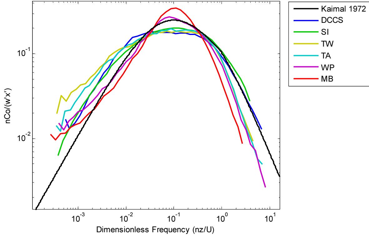
Median wT Unstable Cospectra - 24 May to 12 June 2013
