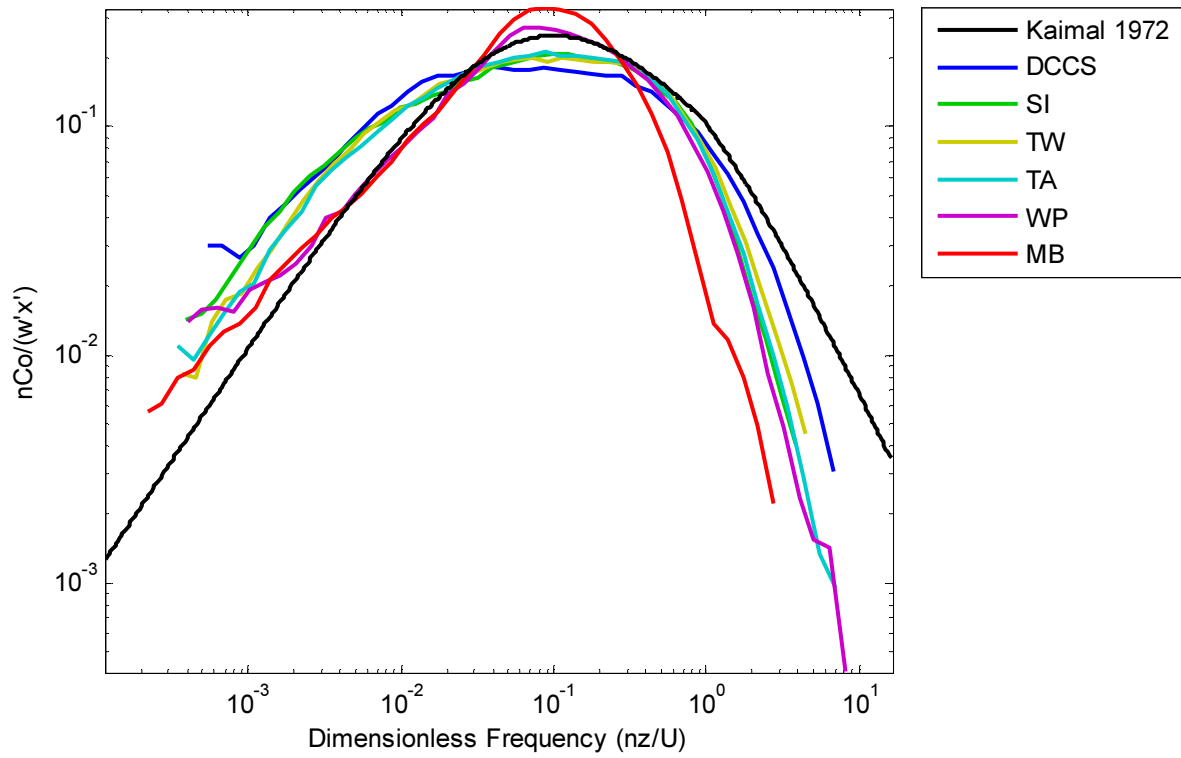
Median wQ Unstable Cospectra - 24 May to 12 June 2013
