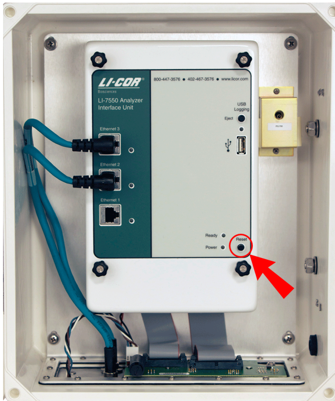
Figure 7-1. Location of Reset button in LI-7550.
