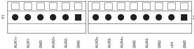
Figure 2-11. Terminal connections for Analog Inputs.
