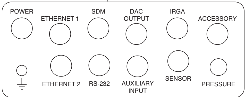
Figure 2-5. LI-7550 Connector Panel.
