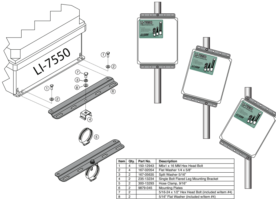
Figure 2-1. Attach mounting plates to Analyzer Interface Unit, attach hose clamp mounting brackets to mounting plates, and secure to mounting post using hose clamps.
