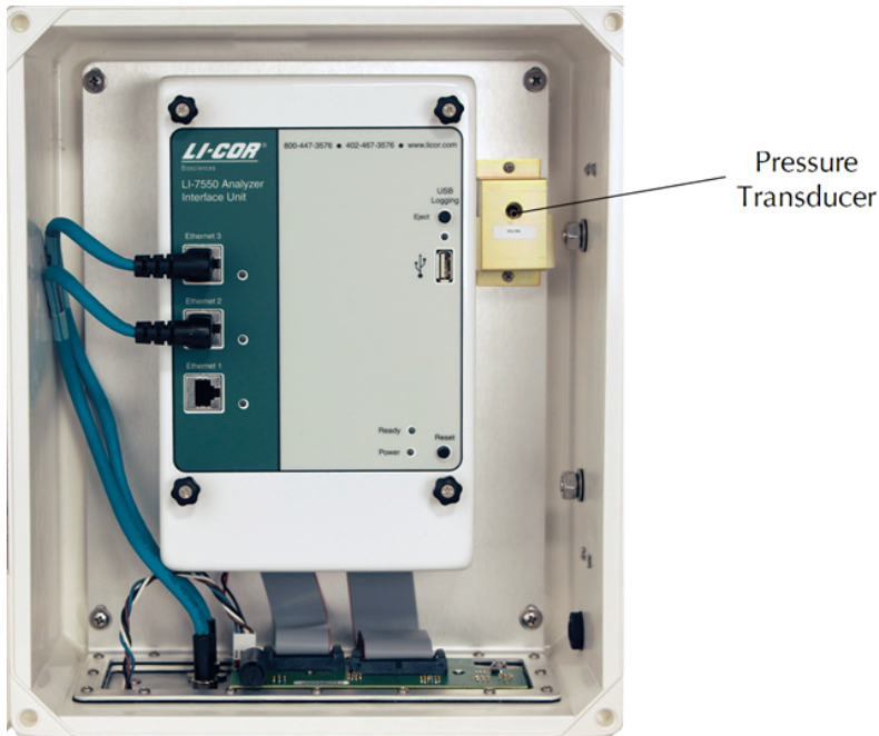
Figure 2-4. LI-7550 indicator panel.
