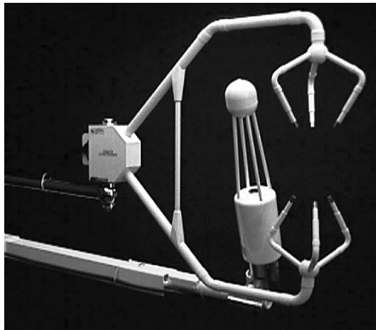
Figure 2-2. Mount the sensor head near the sonic anemometer, at a slight vertical angle.
