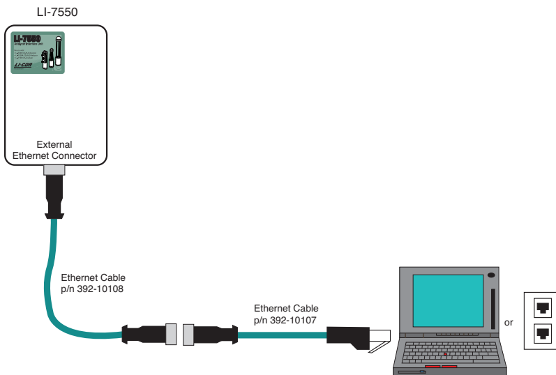
Figure 2-8. Two Ethernet cables are included for connection to an RJ45 connector on a computer or wall socket.
