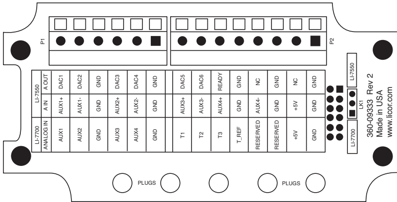
Figure 2-10. Schematic diagram of interior of Auxiliary Interface Box.
