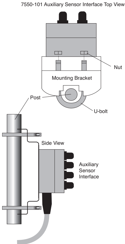
Figure 2-9. Use the included U-bolts and hex nuts to secure the Auxiliary Sensor Interface to a post, if desired.
