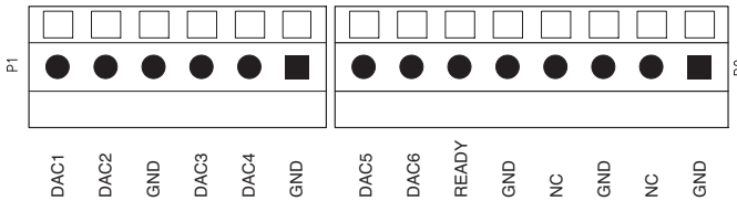
Figure 2-12. Terminal connections for Analog Outputs.
