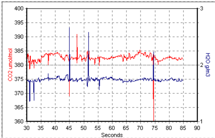
Figure 4-2. Typical strip chart trace taken during a light snow shower.
