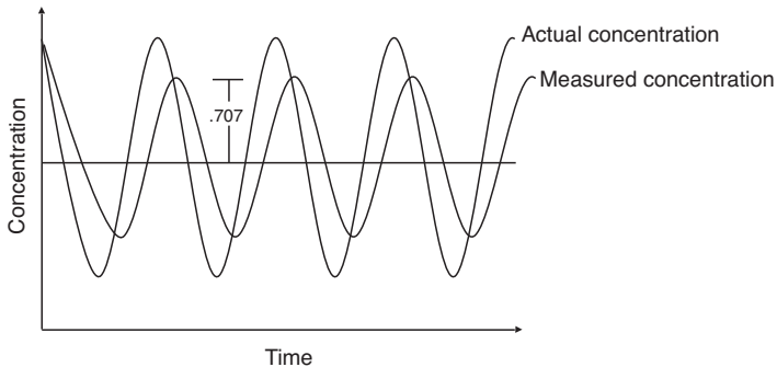
Figure 3-3. Bandwidth = 1/oscillation period.
