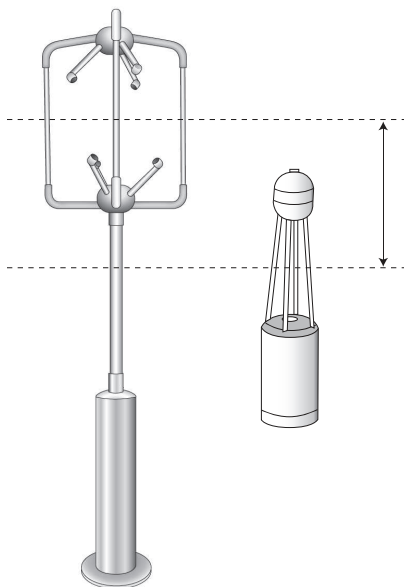
Figure 3-2. Vertical separation of the gas analyzer relative to the sonic anemometer.
