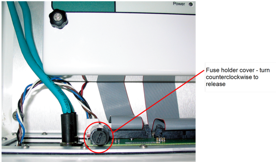
Figure 6-2. LI-7550 fuse location.
