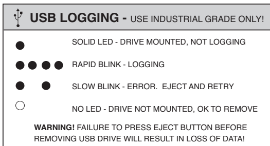
Figure 2-3. This graphic is part of a larger label present on the inside cover of the LI-7550 Analyzer Interface Unit.
