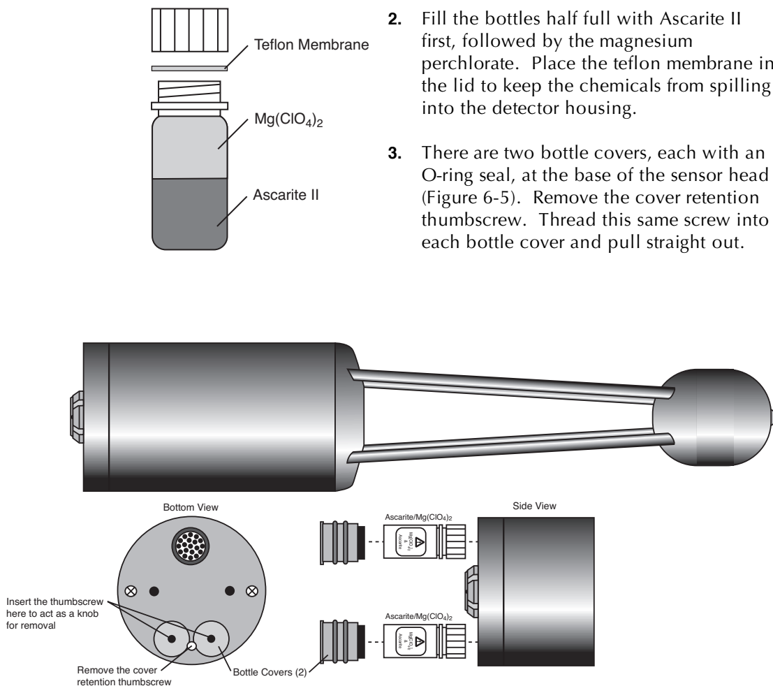
Figure 6-5. Remove the thumbscrew, thread into the bottle covers and replace the chemicals.
