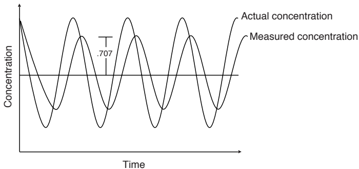
Figure 4-2. \text{Bandwidth} = 1/\text{oscillation period} .
