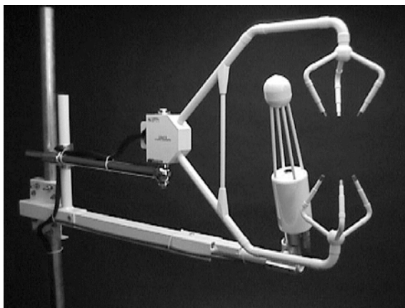
Figure 2-2. Mount the sensor head near the sonic anemometer, at a slight vertical angle.
