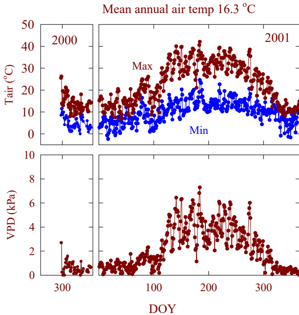
Figure 6 dat of Xu and Baldocchi. Annual grassland near Ione Cal
